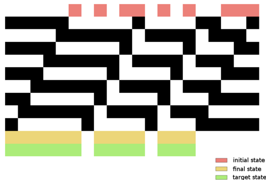
Figure 2. Successful attempt at solving a research problem. A certain rule (scientific method) is applied to an initial state (red) for a certain amount of time steps (here: 10). The final state (yellow) matches the target state (green) perfectly, indicating complete success.
