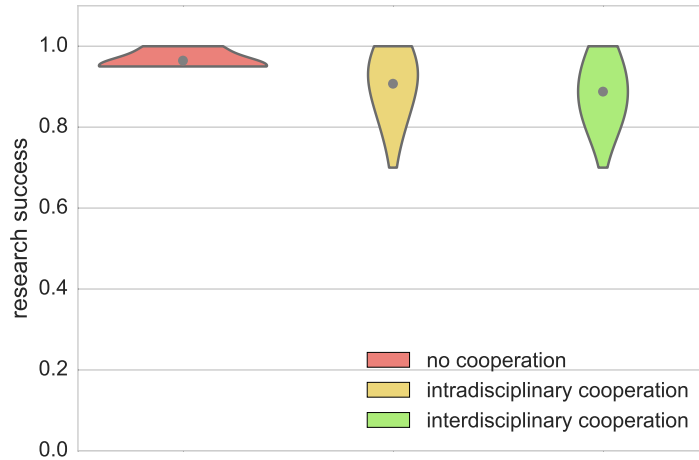
Figure 8. Success rate for solving medium research problem (20 cells), when the solution to a similar problem is already known. In this scenario, the non-cooperative strategy outperforms all other strategies, since changing the used research method due to cooperation is a disadvantage in this case.
