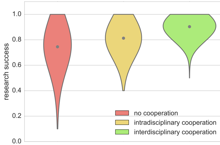
Figure 5. Success rate for solving simple research problems (10 cells). Here, interdisciplinary cooperation is more successful than the other strategies. The non-cooperative strategy performs worst.
