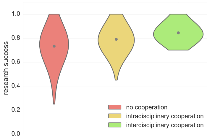
Figure 6. Success rate for solving medium research problems (20 cells). The situation is similar to the one for simple problems, the differences between strategies are, however, less pronounced.
