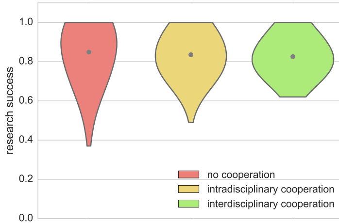
Figure 7. Success rate for solving difficult research problems (100 cells). Here, the non-cooperative strategy performs best on average and has the most 100% successful attempts.
