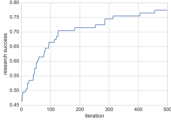
Figure 3. Proximity development during iterative research process. The proximity is increasing monotonically, but P = 1 is not necessarily reached within 500 iteration steps.
