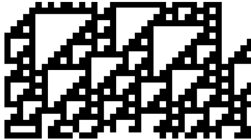
Figure 1. Time development of an arbitrary state using rule 110. Each line represents a discrete time step in this time development, with time running from top to bottom. In this visualization the complex nature of the arising patterns is clearly visible.
