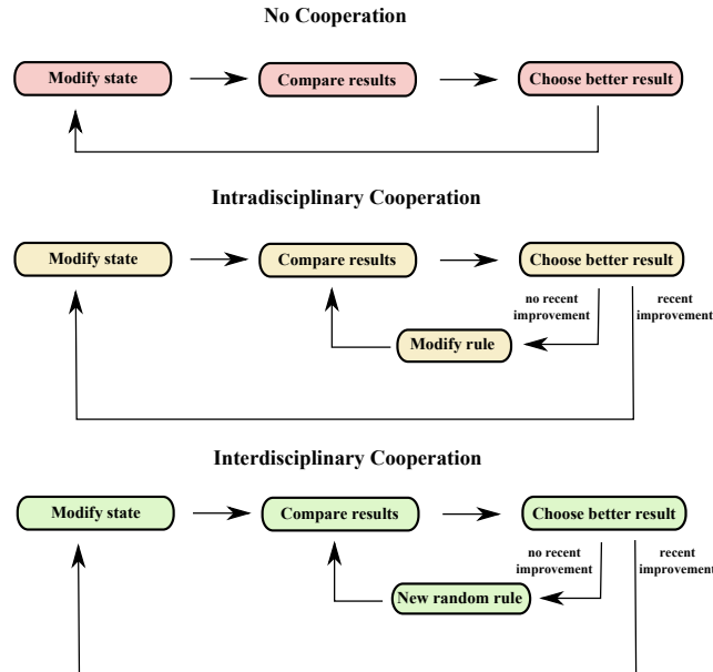
Figure 4. Modeled research process for different research strategies. While non-cooperative research stays with the initial method, cooperative research can lead to modifications or changes of the used method.
